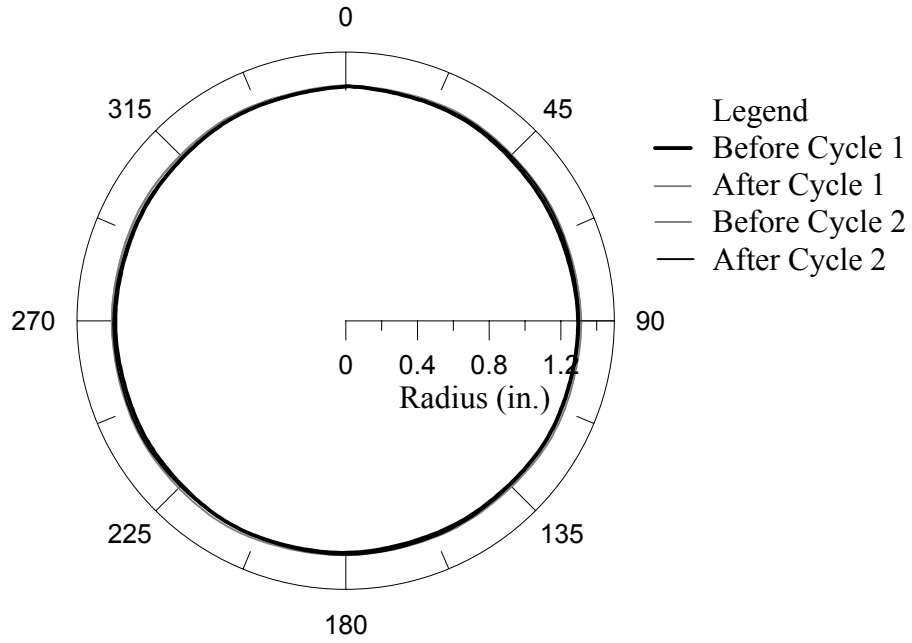
Fig. 78: Surface-deformation plot for 5.0-inch band for PD05
