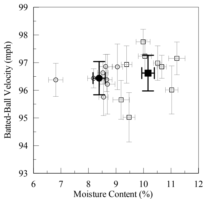
Fig. 81: Measured AEV from sweet spot as function of moisture content
