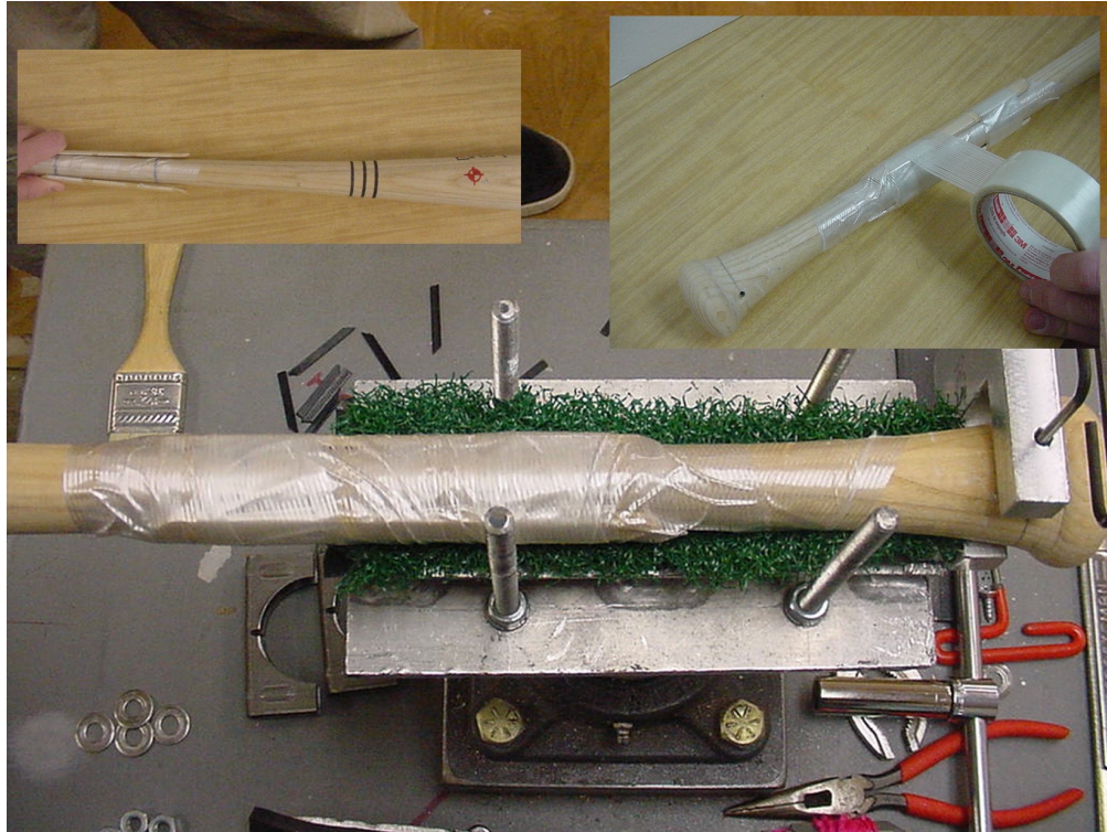
Fig. 16: Wrapping of handle of wood bat for reinforcement
