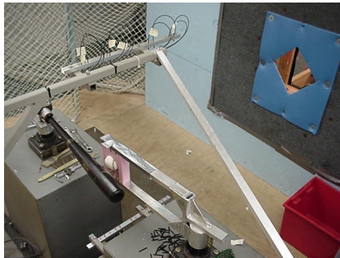
Fig. 4: View of BHM in UMLBRC from top corner
