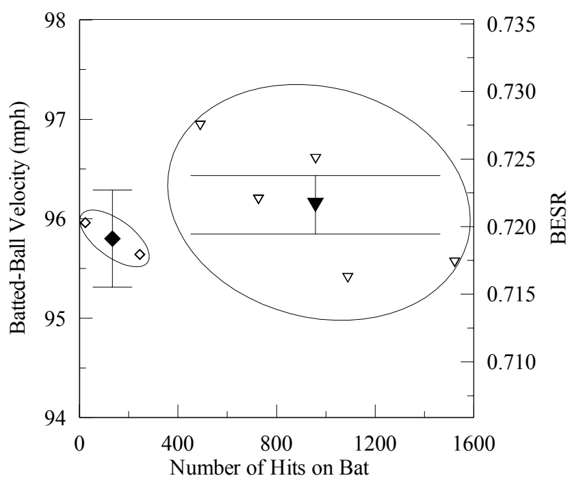
Fig. 70: Analysis of lumped BESR-based AEV for 5.0-, 5.5- and 6.0-inch locations for PD04
