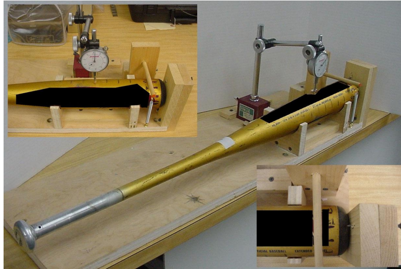
Fig. 12: Surface deformation setup
