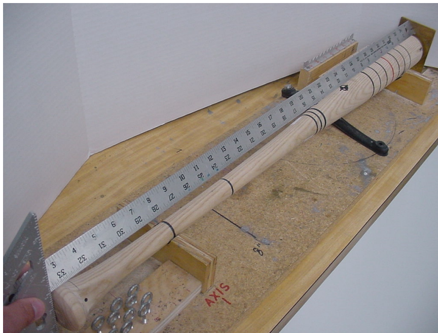
Fig. 7: Use of carpenter's square with profiling station
