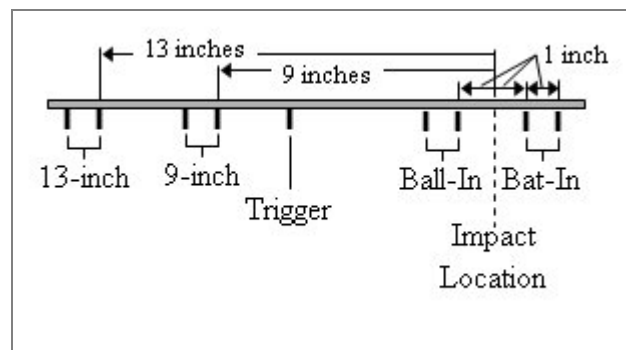
Fig. 5: Diagram of photoelectric sensors in BHM
